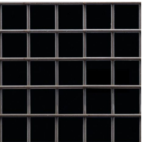
MTL-1 WIRE MESH MFR: MCNICHOLS WIRE MESH PRODUCT: SQUARE CARBON STEEL SIZE: 70% OPEN SQUARE MESH
