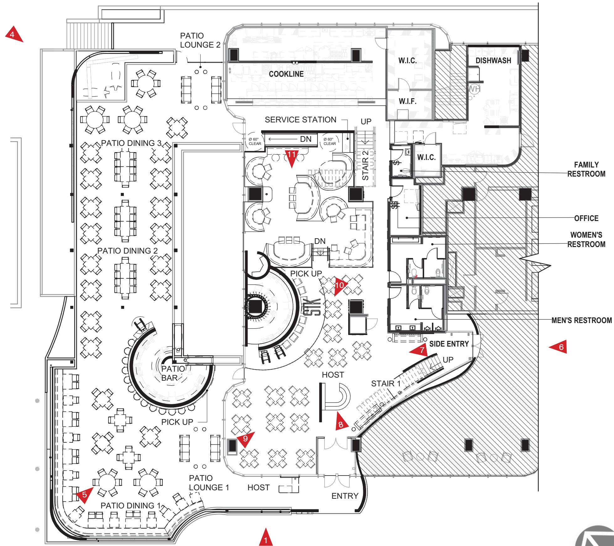
Plaza Floor Plan
