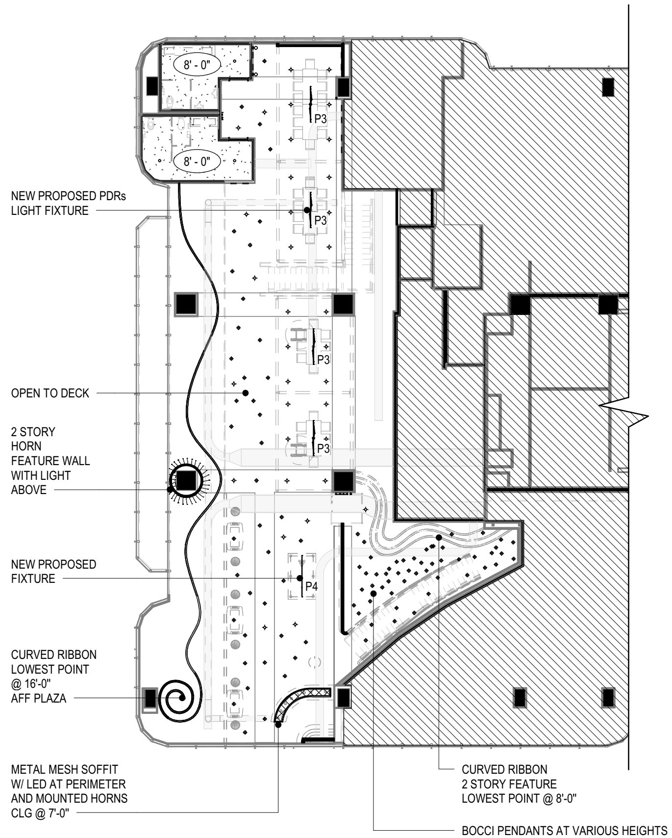
Mezzanine Reflected Ceiling Plan
