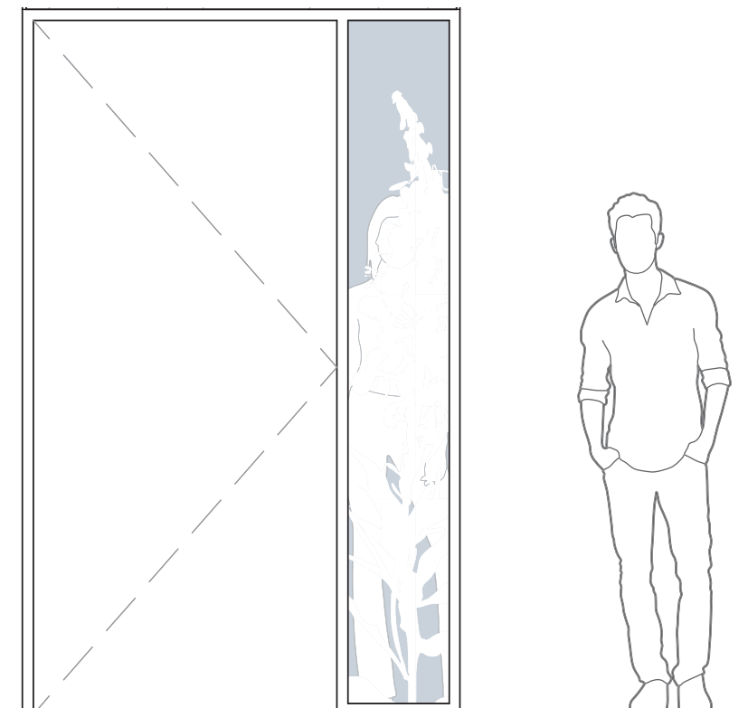
2 ELEVATION: MEDITATION ROOM GLASS FILM (DISTRACTION) SCALE: 1/2" = 1'-0"
